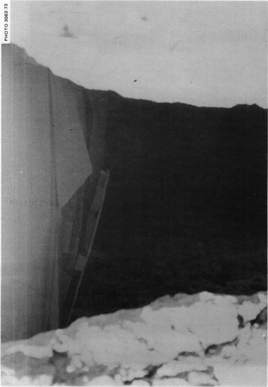
Fig. 3.6. Looking into the shelter after the rupture of the lower plywood-veneer sides of the doors. Since the veneer on the upper sides of the two partially broken doors and of two cracked doors remained intact, no earth fell into the shelter, and occupants would not have been injured by this unexpected type of failure of the most stressed of these very light hollow-core interior doors used for trench roofing.
